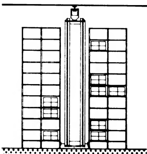
17 Possibilities for fixing guide rails: guide rails above
